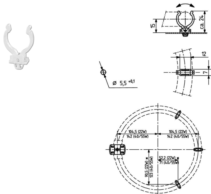
Example of application (Sheet metal layout)
